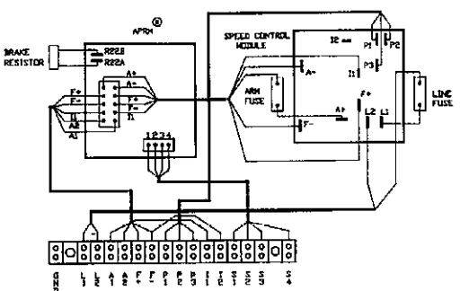
FIG. 5 INTERNAL CONNECTION DIAGRAM
