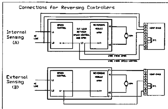
FIG. 5 INTERNAL CONNECTION DIAGRAM
