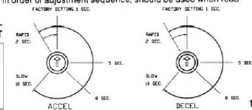
Fig. 4 ACCEL/DECEL TRIMPOT ADJUSTMENT
